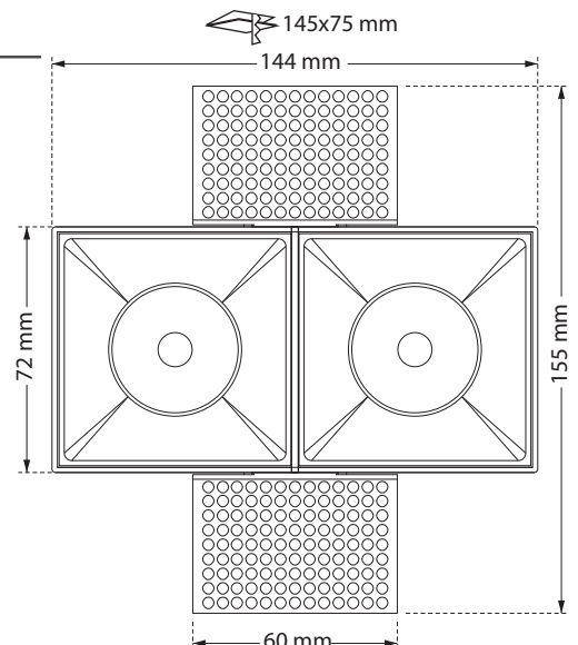
Honey comb louvre
